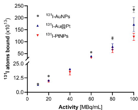
Fig. 2 Surface saturation of AuNPs, Au@Pt NPs and PtNPs with 10–100 MBq \text{mL}^{-1} ^{131}\text{I} ( n = 3 ).
